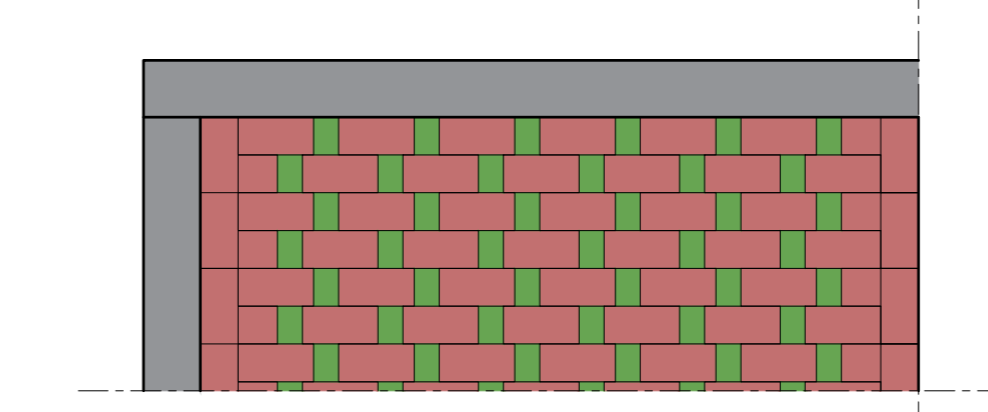
Detail open bestrating Schaal 1:20
